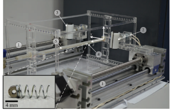
Fig. 2. A magnetic-based robotic system for the motion control of a helical robot (inset). The system consists of two synchronized linear motion stages (1). Each stage holds a rotating permanent magnet (2 and 3) to actuate the helical robot (4). The rotating permanent magnets are also synchronized using a control system. The helical robot is contained inside a glass tube (5) with inner diameter of 10 mm. The synchronized rotation of the rotating permanent magnets allows us to eliminate the attractive components of the magnetic force on the magnetic dipole of the helical robot. The diameter, length and wire diameter of the helical robot are 4 mm, 12.5 mm, and 0.7 mm, respectively.
