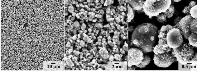
Fig. 2. Scanning electron micrographs of iron oxide nanoparticles. The maximum diameter of the nanoparticles is approximately 2 \mu\text{m} . These nanoparticles are pulled under the influence of a magnetic field gradient towards the MCF-7 cells to achieve immediate and selective uptake. The magnetic dipole moment of a cluster with a mass of 1.8 \times 10^{-9} \text{ kg} is calculated to be 7.8 \times 10^{-8} \text{ A}\cdot\text{m}^2 , and the magnetic force exerted on this dipole is measured to be 0.39 \mu\text{N} under the influence of magnetic field gradient of 5 \text{ T}\cdot\text{m}^{-1} . The magnetic field is measured using a 3-axis digital Teslometer (Senis AG, 3MH3A-0.1%-200mT, Neuhofstrasse, Switzerland), and the magnetic field gradients are calculated numerically.
